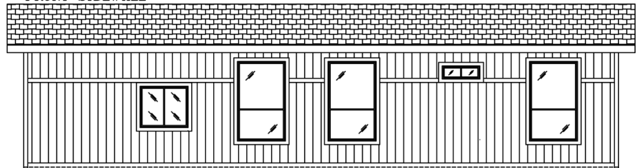
BACK SIDEWALL
